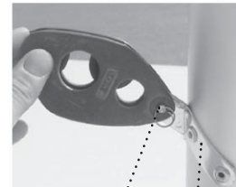
figure 66 | cleat, vang tang
