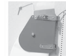
figure 76 | rudder downhaul line
